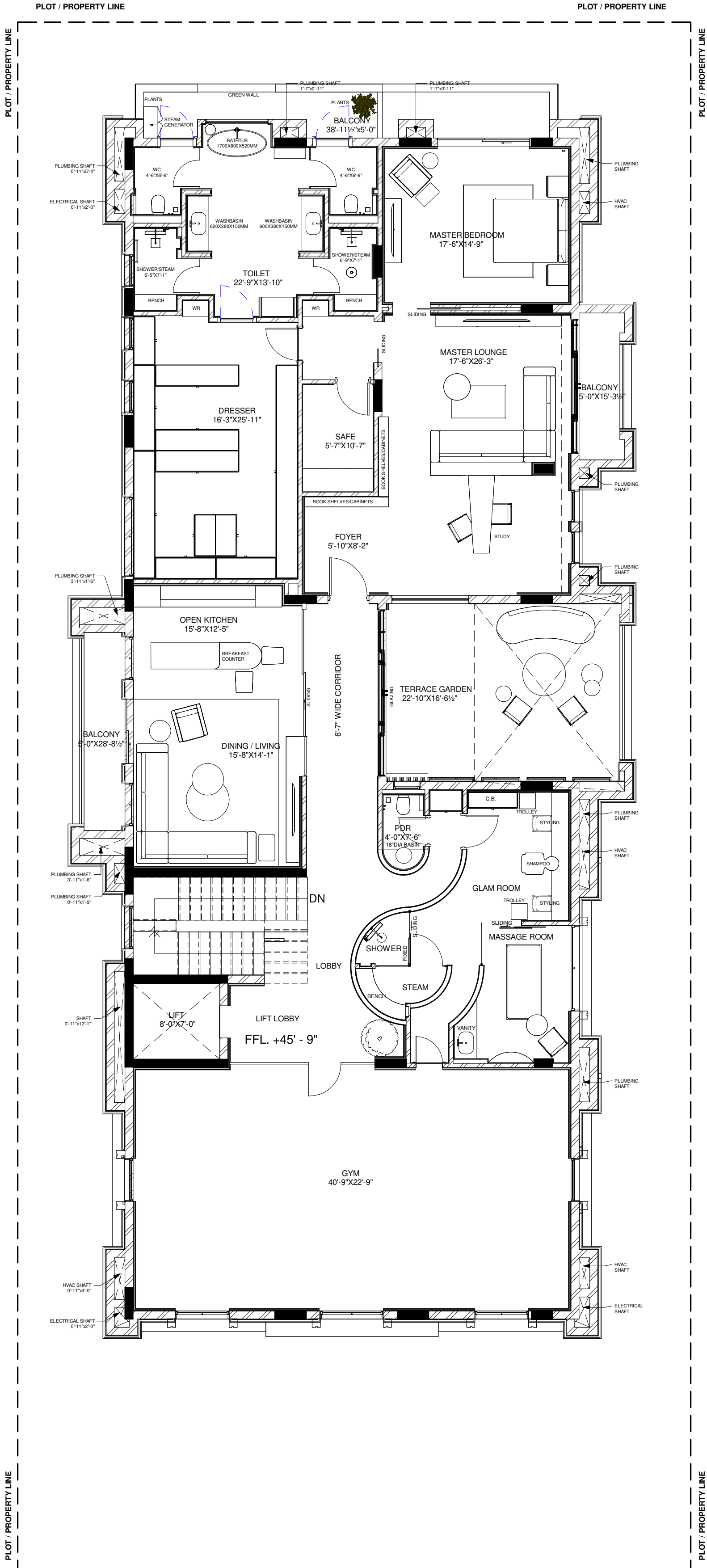
1 Third floor layout 1/8" = 1'-0"
